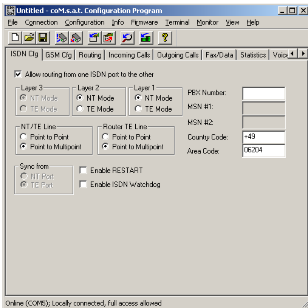
Figure 36: Router Configuration
