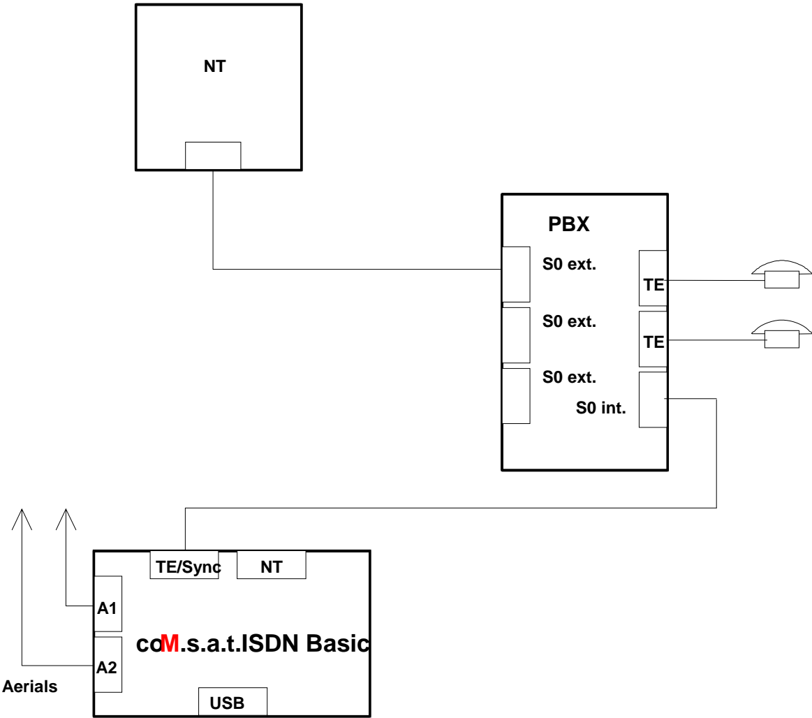
Figure 33: TE Installation
