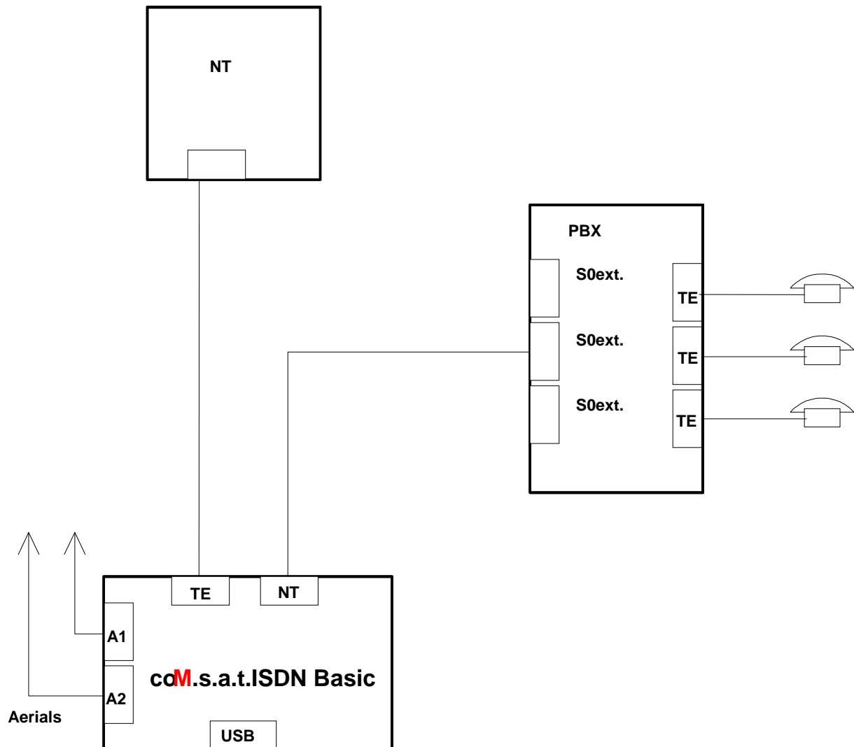
Figure 35: Router Installation
