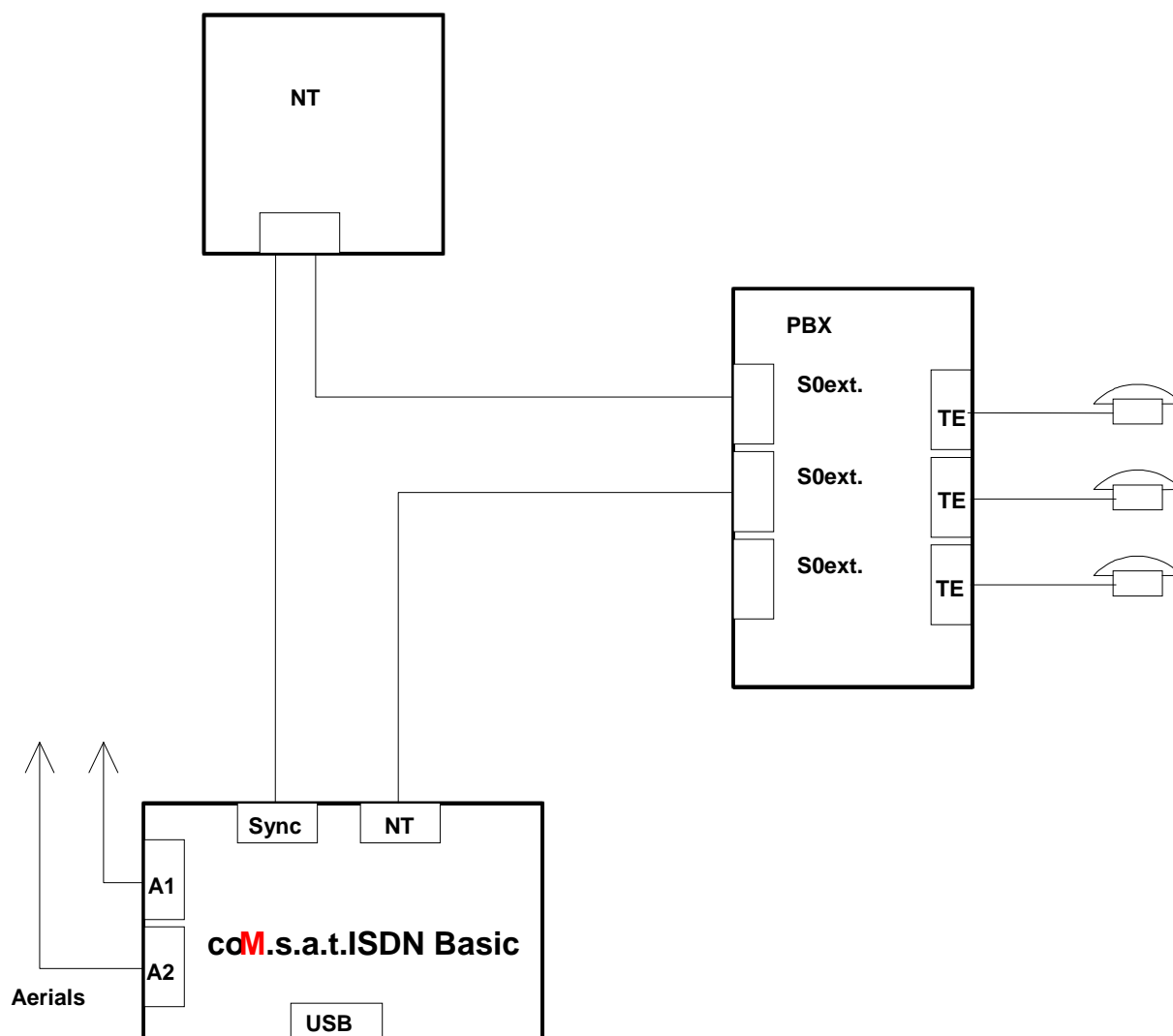
Figure 31: NT Installation
