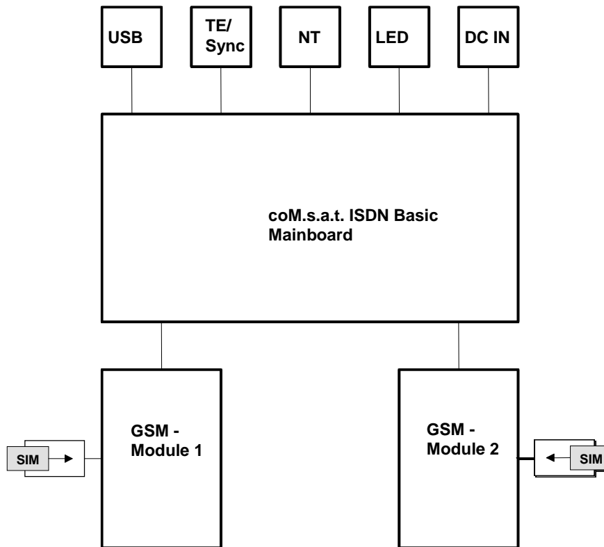
Figure 1: Functional Groups
