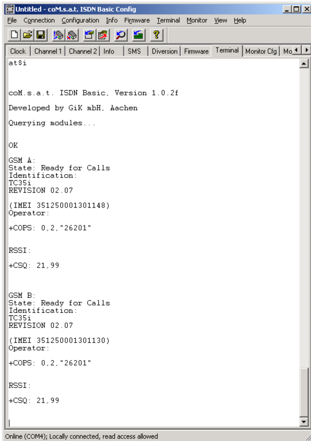
Figure 22: Module information in the terminal window
