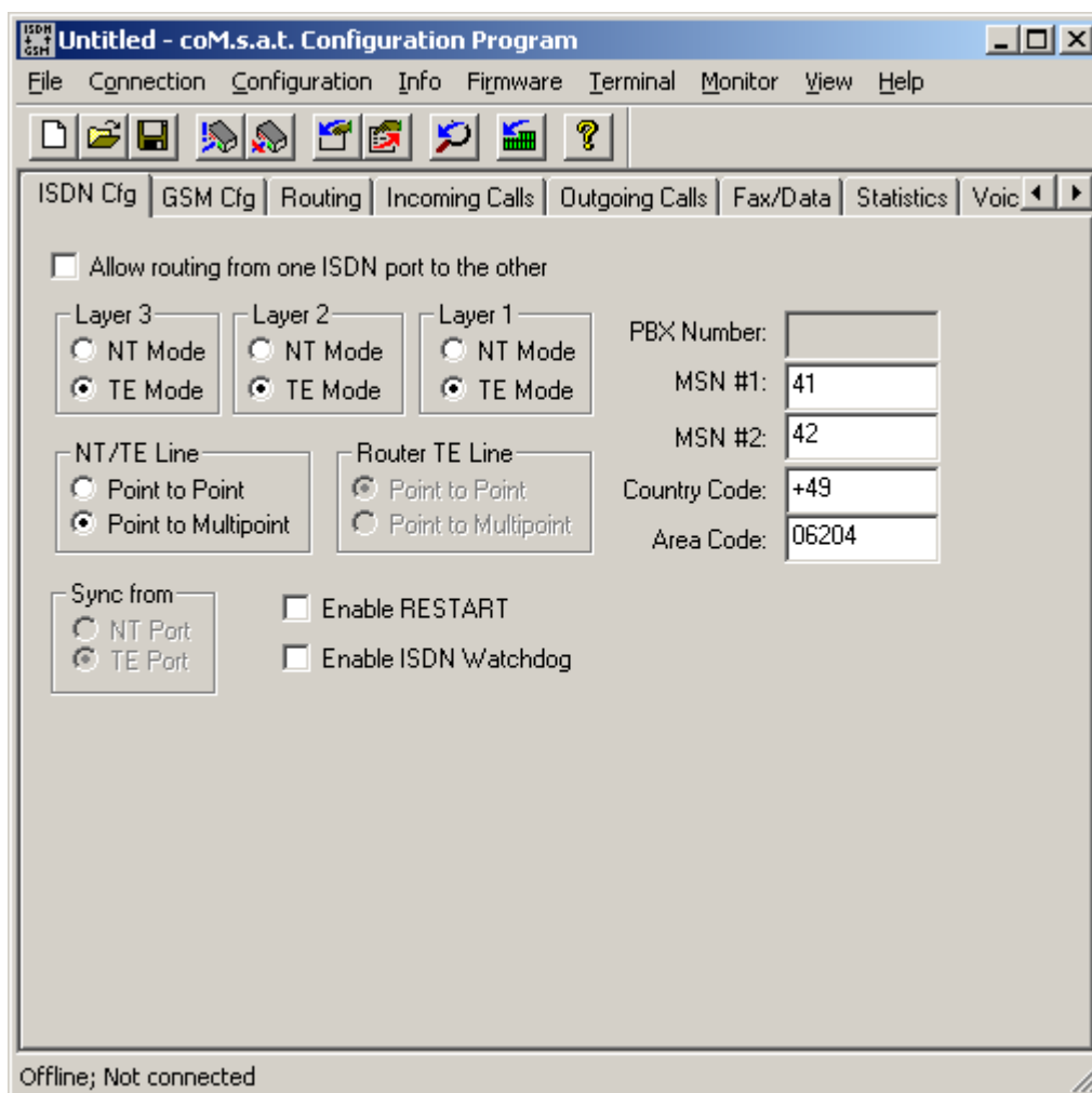
Figure 34: TE Configuration
